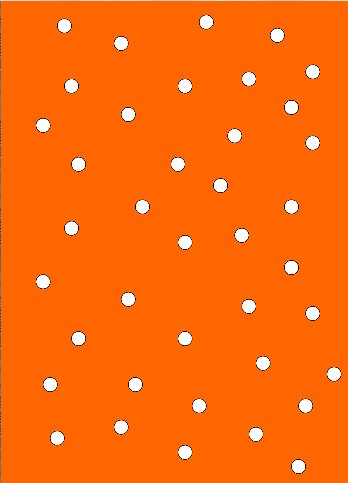
Diagram #2 Less Dense, Warm Air or Water Molecules (Land)
